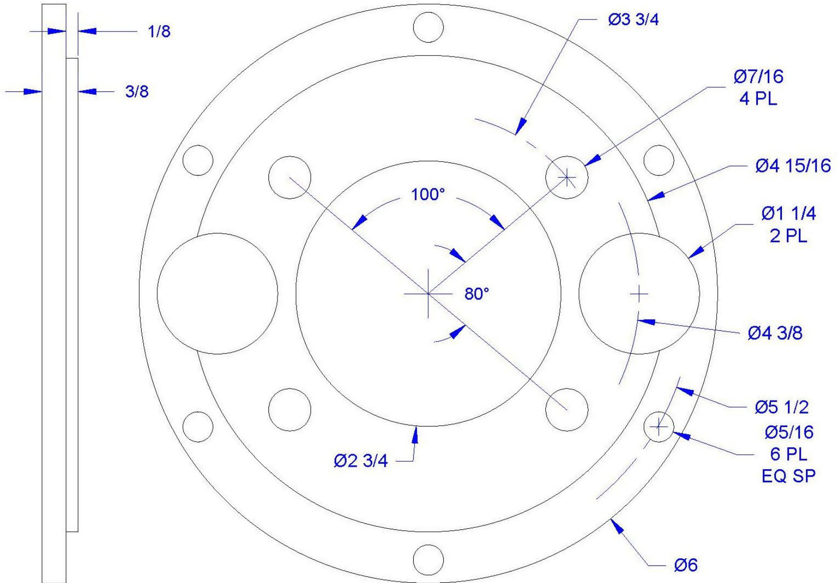
HUB FOR VENTED REAR BRAKE ROTOR
